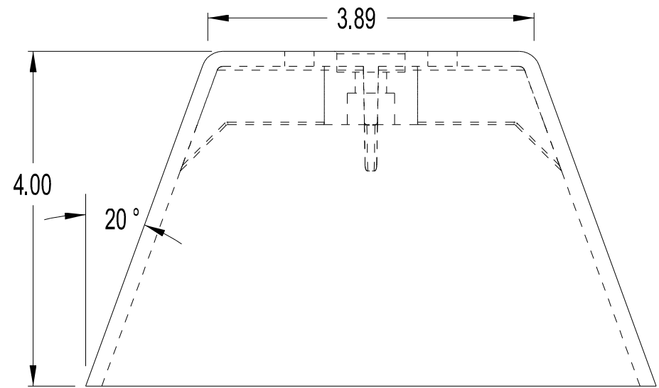
TANK ADAPTER PLUG MANDRELS PART # 3010 MATERIAL - FILLED POLYPROPYLENE
