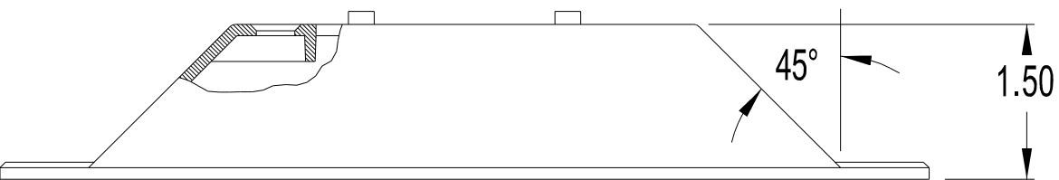
PL-122 BR ADAPTER PART NO. - 30144 MATERIAL- POLYPROPYLENE
